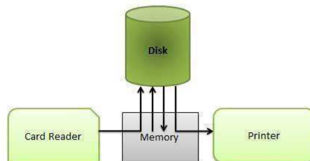
Fig 1.5 Spooling
