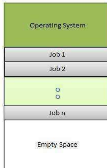
Fig 1.4 Multiprogramming
