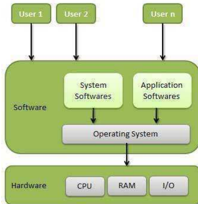
Fig 1.1 Operating System
